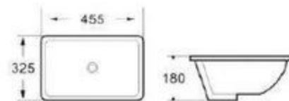
UNDER COUNTER WASH BASIN
